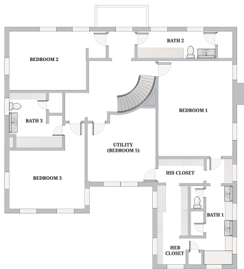
UPPER LEVEL
